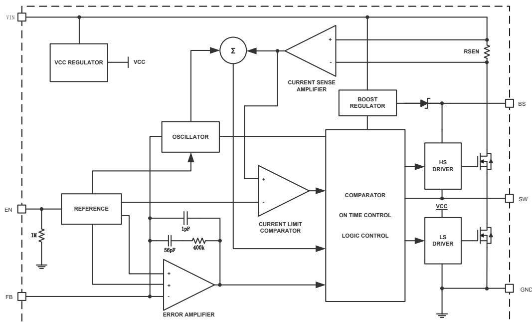
Figure 2. HM1482E Block Diagram
