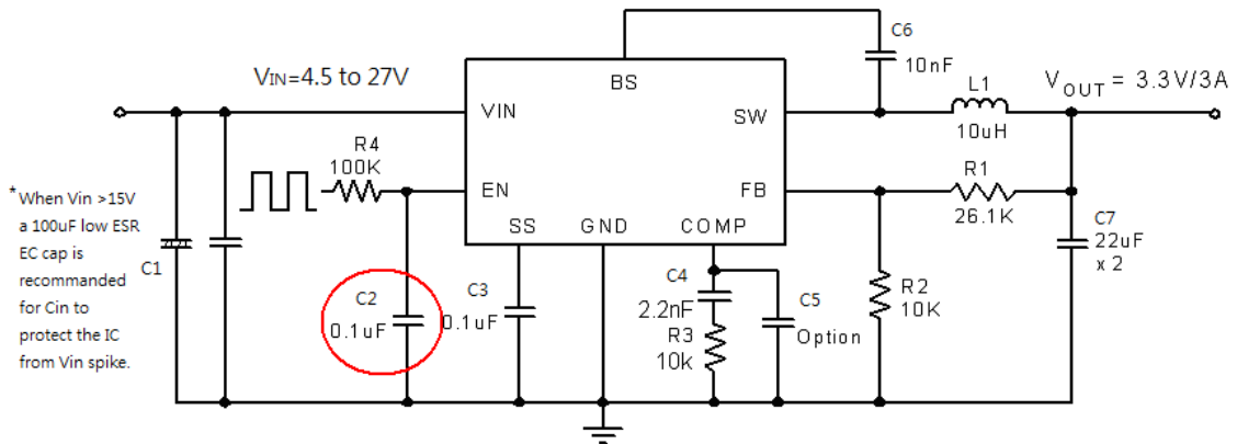
< A%, ( 5 application circuit, 3.3V/3A output with EN function
