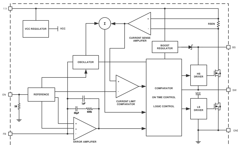
Figure 2. HM1484D Block Diagram
