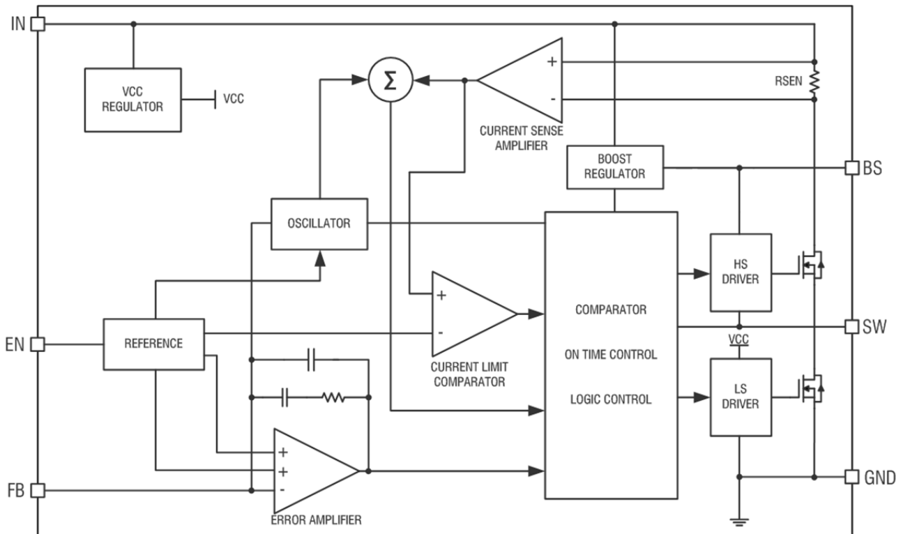
Figure 2. HM1484F Block Diagram
