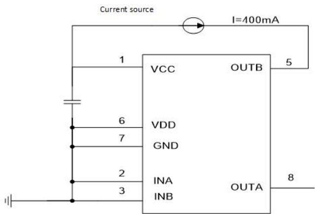
PMOS body diode conduction voltage test schematic
