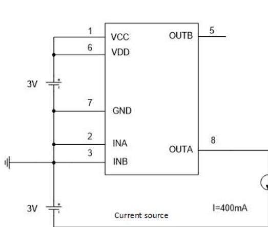
NMOS body diode conduction voltage test schematic
