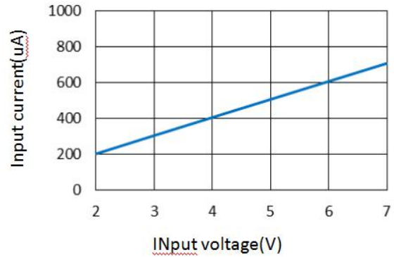
The logic input current varies with the voltage curve
