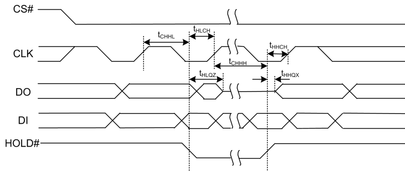
Figure 8.6 Hold Timing
