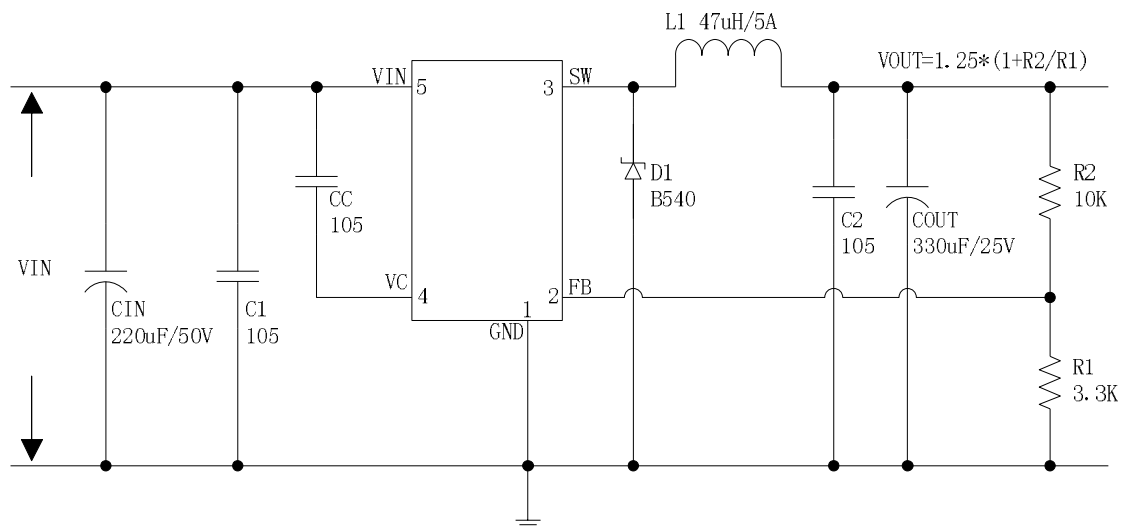
Figure4. HM3105 Typical Application Circuit ( V_{IN}=8V\sim36V , V_{OUT}=5V/5A )
