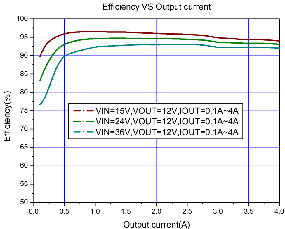
Figure8. HM3105 System Efficiency Curve
