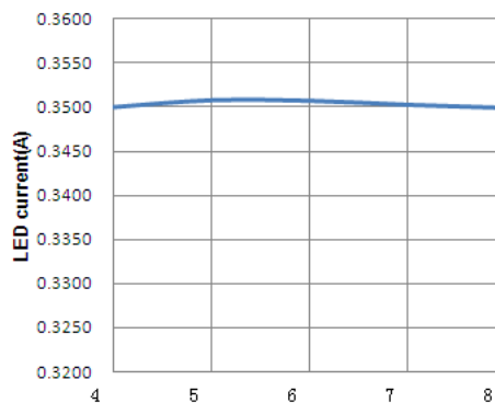
LED 电流 VS. 输入电压(3 颗 LED)
