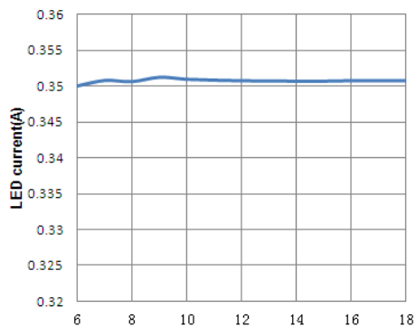
LED 电流 VS. 输入电压(6 颗 LED)
