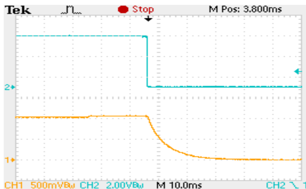
Shutdown Waveform
