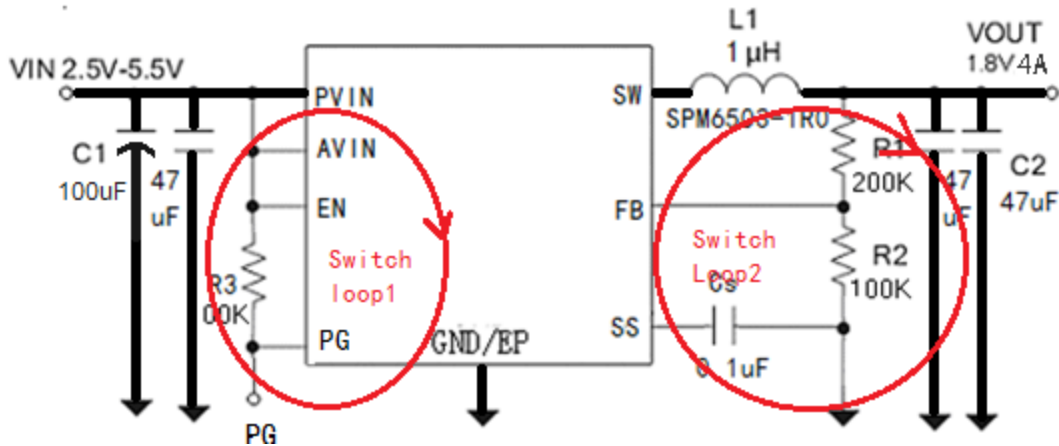
Big Current Circuit & Switching Loop
