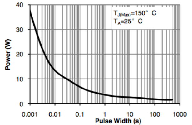
Figure 10: Single Pulse Power Rating Junction-Ambient (Note E)
