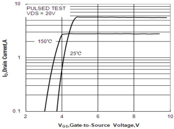
Figure 6 Typical Transfer Characteristics
