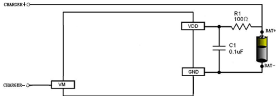
Fig 6 HM5431S in a Typical Battery Protection Circuit
