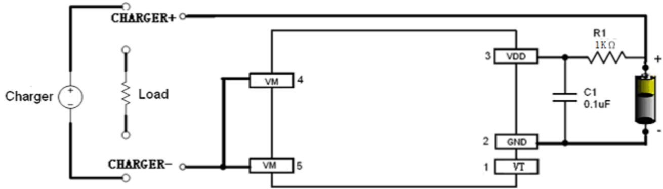
Fig 6 <A) (%) % in a Typical Battery Protection Circuit
