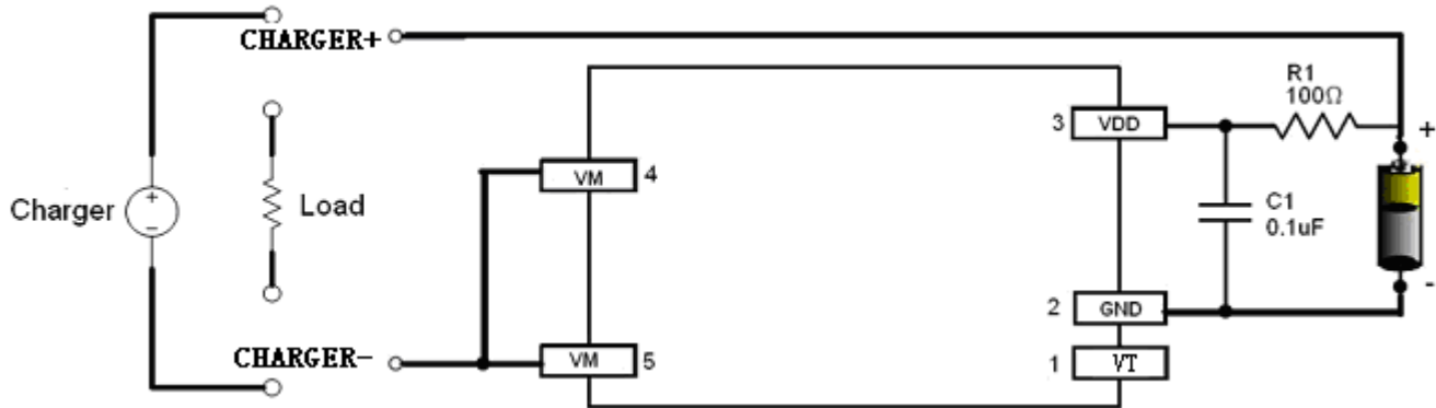
Fig 6 HM5453 in a Typical Battery Protection Circuit
