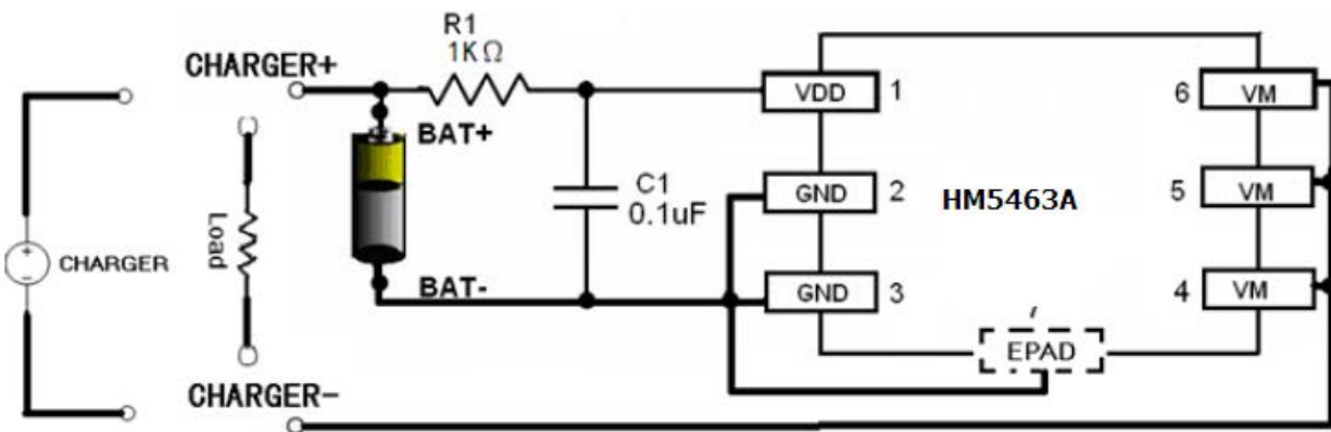
Fig 6 HM5463A in a Typical Battery Protection Circuit
