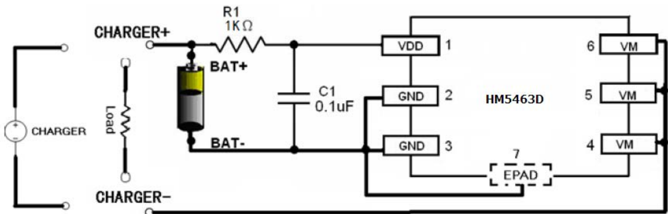
Fig 6 HM5463D in a Typical Battery Protection Circuit
