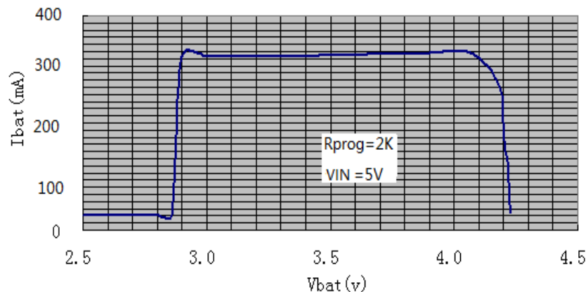
Battery charger curve
