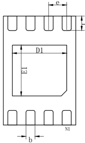
bottom view
