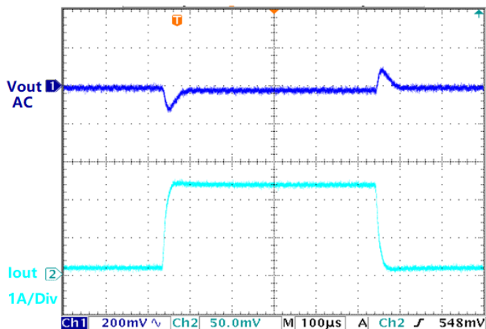
Transient Waveform(Iout=0.15A-1.5A)
