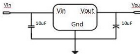
Application circuit of HM7110 fixed version
