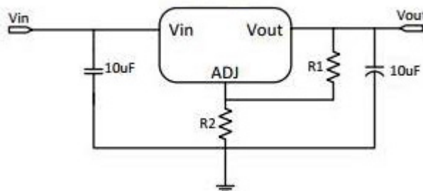
Application Circuit of HM7110-ADJ
