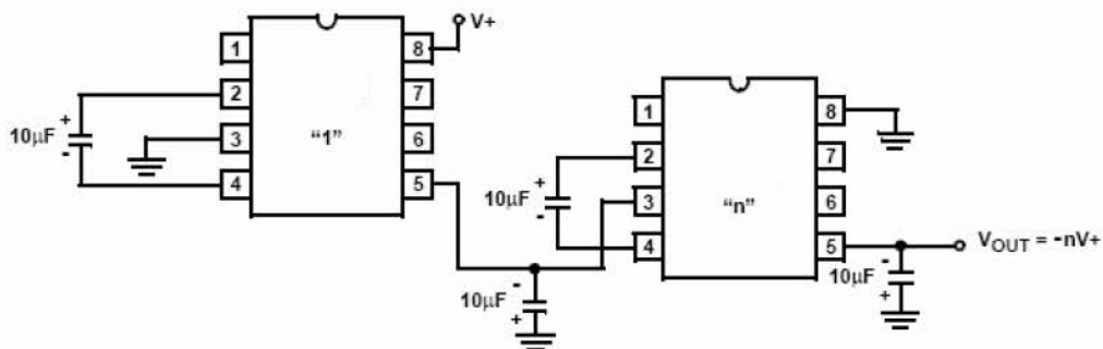
FIGURE 3. CASCADING DEVICES FOR INCREASED OUTPUT VOLTAGE
