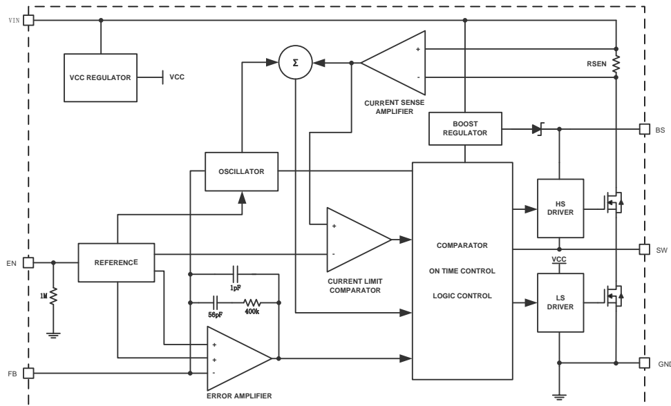
Figure 2. HM8112 Block Diagram
