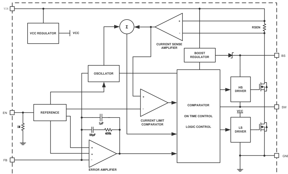
Figure 2. HM8114 Block Diagram
