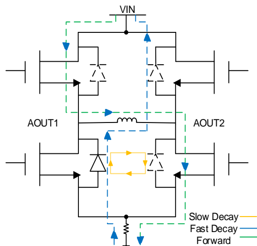
Figure2: Forward Operation
