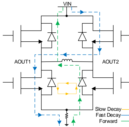
Figure3: Reverse Operation
