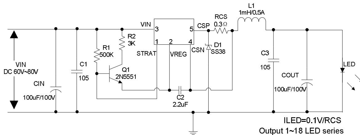
Figure7. HM9802 System Application at VIN=60V~80V Schematic
