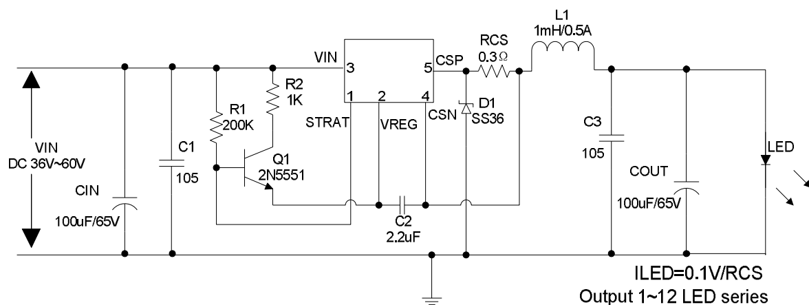
Figure9. HM9802 System Application at VIN=36V~60V Schematic
