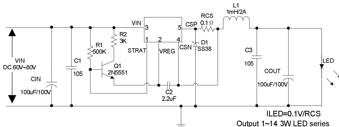
Figure13. HM9802 System Application at VIN=60V~80V Schematic
