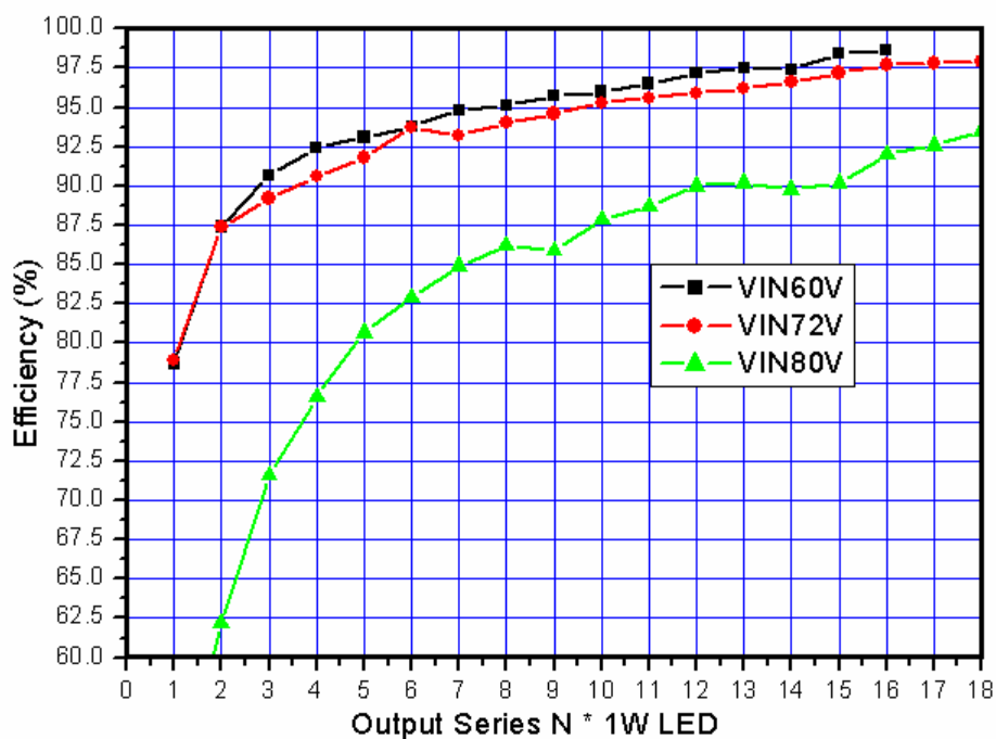
Figure8. HM9802 System Application at VIN=60V~80V Efficiency Curve
