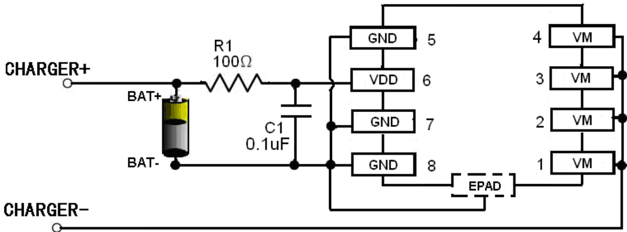
Fig 6 HM9902C in a Typical Battery Protection Circuit
