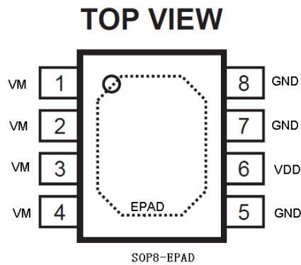
Figure 2. PIN Configuration
