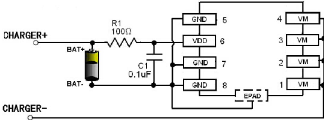
Fig 6 HM9902D in a Typical Battery Protection Circuit
