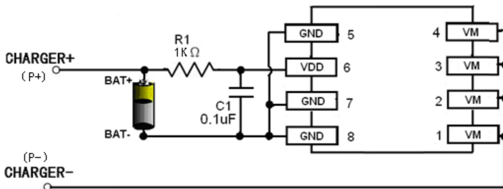
Fig 6 HM9904G in a Typical Battery Protection Circuit
