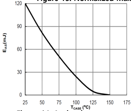
Figure 14: Avalanche energy
