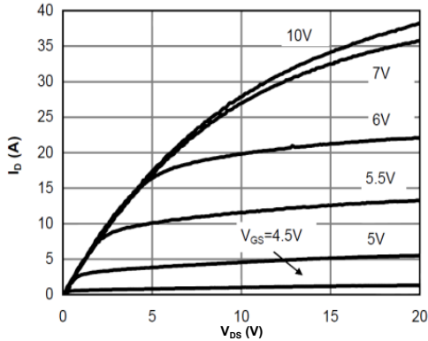
Figure 1: On-Region Characteristics@25°C
