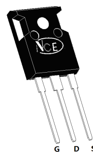
TO-247
