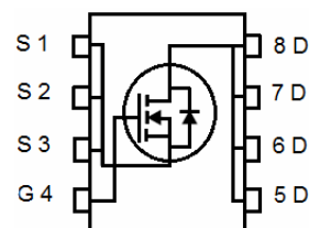
Schematic Diagram
