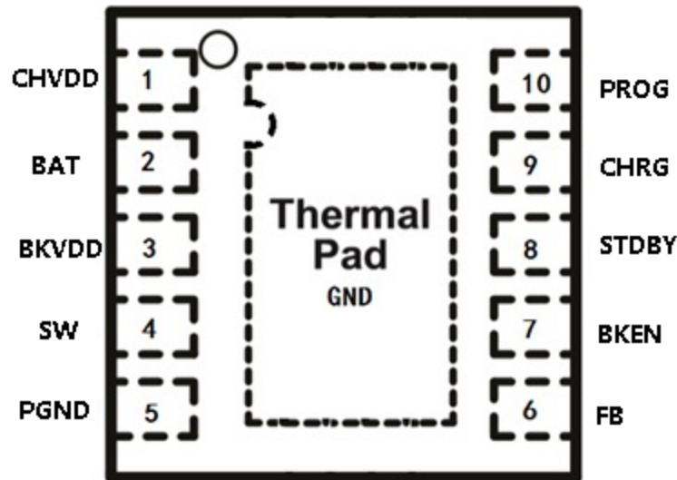
Figure 2. PIN Configuration
