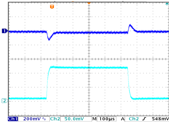
Transient Waveform(Vout=3.3V,Iout=0.15A-1.5A)
