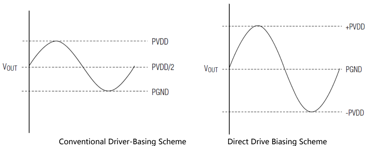
Fig. 1 Conventional Driver Output Waveform vs. HM97220 Output Waveform
