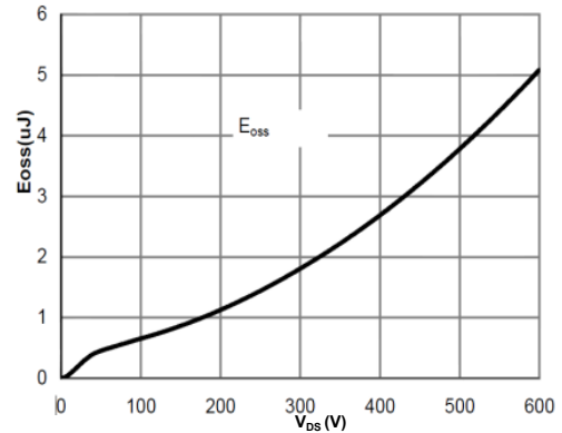
Figure 10: C oss stored Energy
