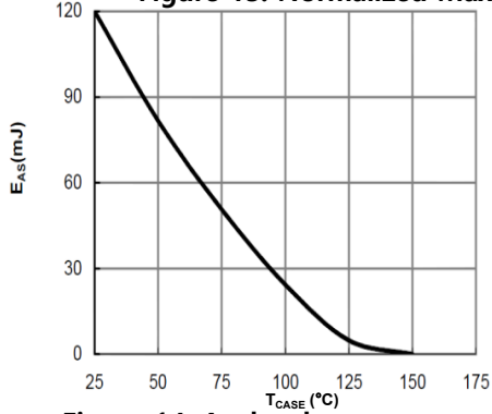
Figure 14: Avalanche energy
