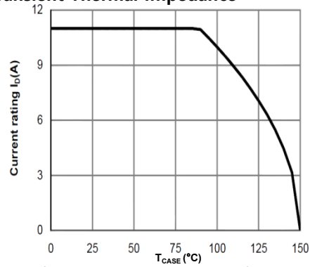
Figure 15: Current De-rating
