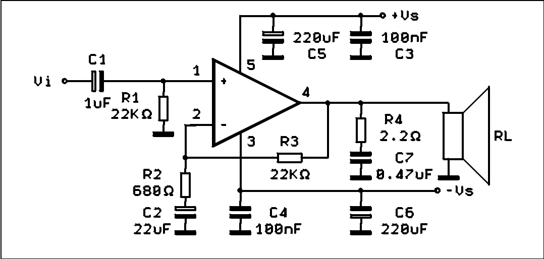
Figure 4. Split-supply typical application circuit
