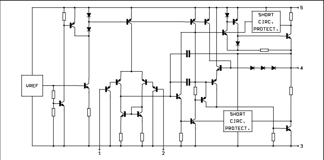
Figure 3. Schematic diagram
