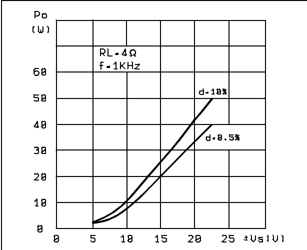
Figure 10. Output power vs. supply voltage
